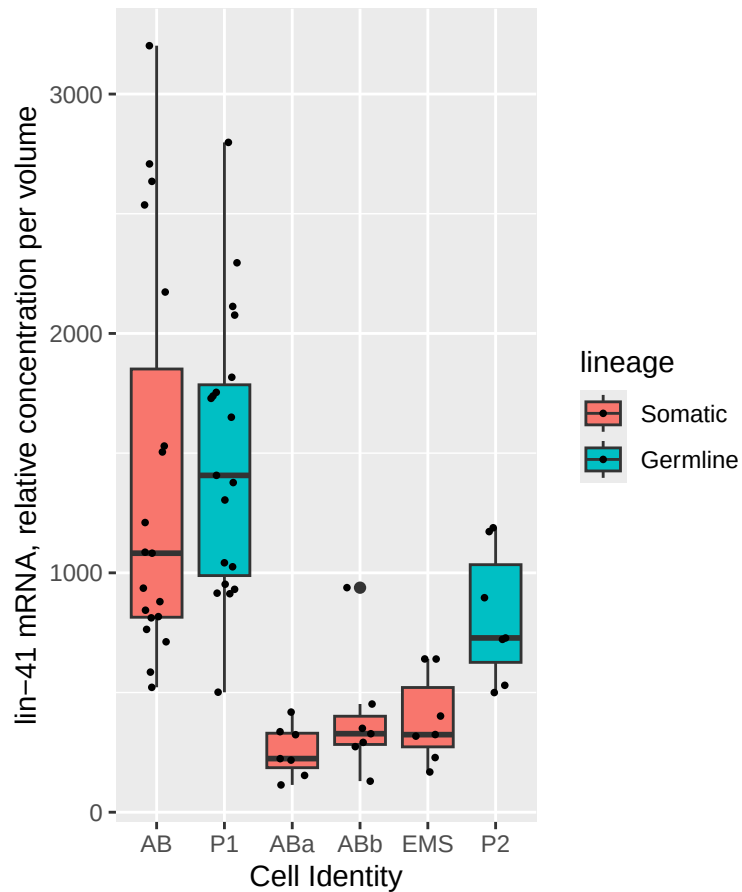
lin-41 mRNA, relative concentration
