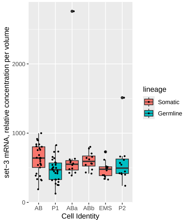
set-3 mRNA, relative concentration
